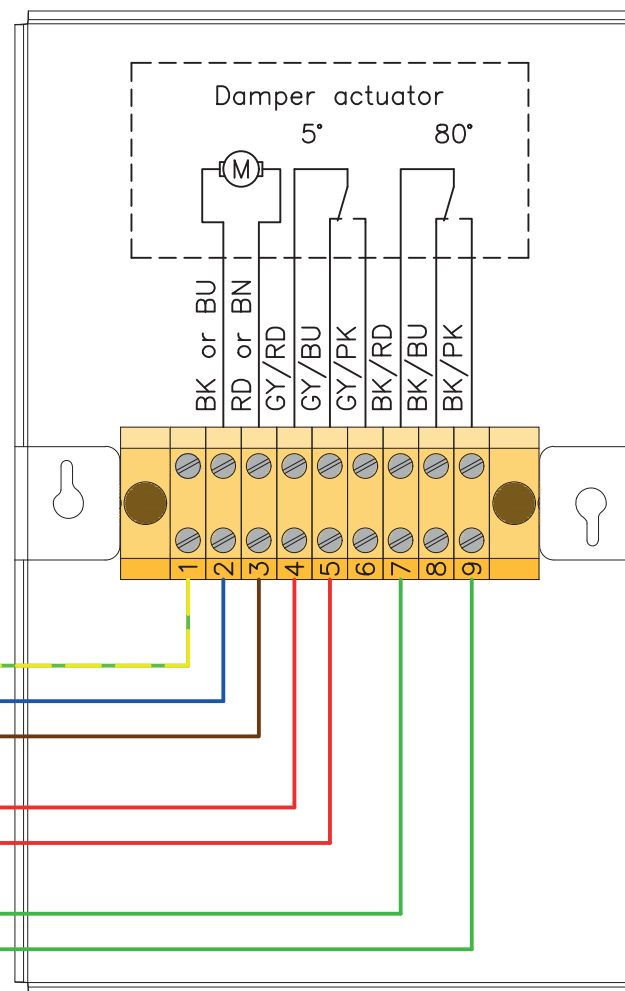
Damper junction box
