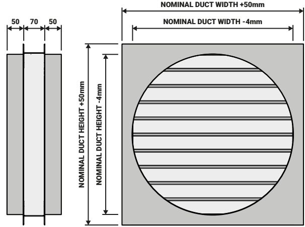
1400 Dimensions – Circular Spigot
