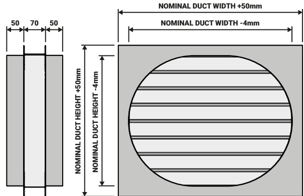
1400 Dimensions – Flat Oval Spigot
