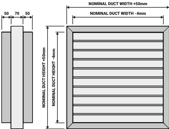
1400 Dimensions – Rectangular Spigot
